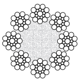
8 x 19 Seale
