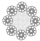
8x19 Seale CompactTrac™
