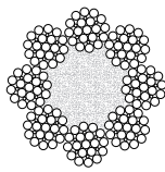
8 x 25 Filler Wire
