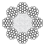
8 x 19 Warrington
